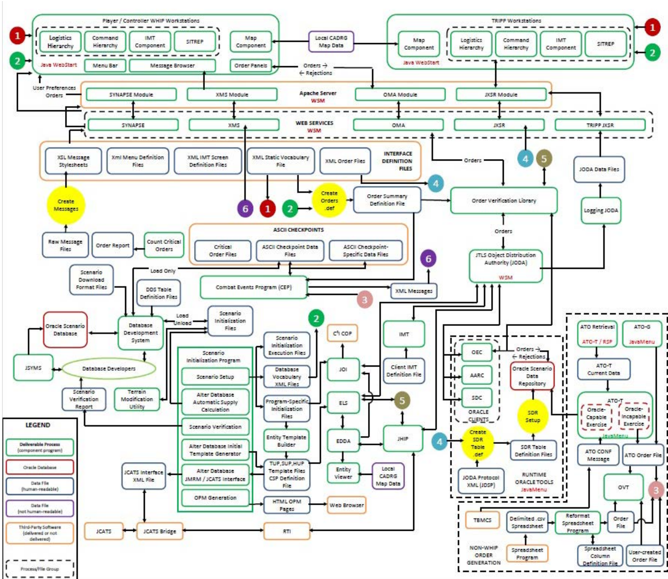
Figure 4.1 Web Enabled JTLS-GO System Structure And Data Flow
