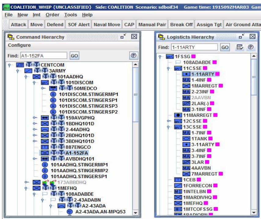
Figure 4.4 Command Hierarchy And Logistics Hierarchy Windows
